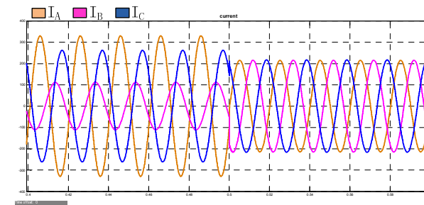
(c) Current of tractive transformer high voltage side( \frac{2}{3} \leq Y \leq 1 )
