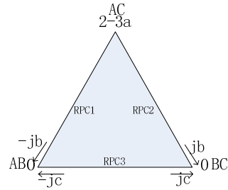
(c) Reactive power compensation based on Steinmetz theory
