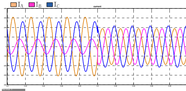
(b) Current of tractive transformer high voltage side( 0 \leq Y \leq \frac{2}{3} )
