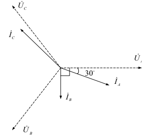
Figure 2. Three-phase current phase diagram without compensation
