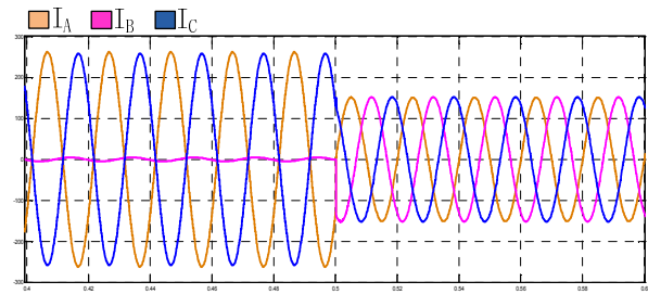
(a) Current of tractive transformer high voltage side( Y=0 )
